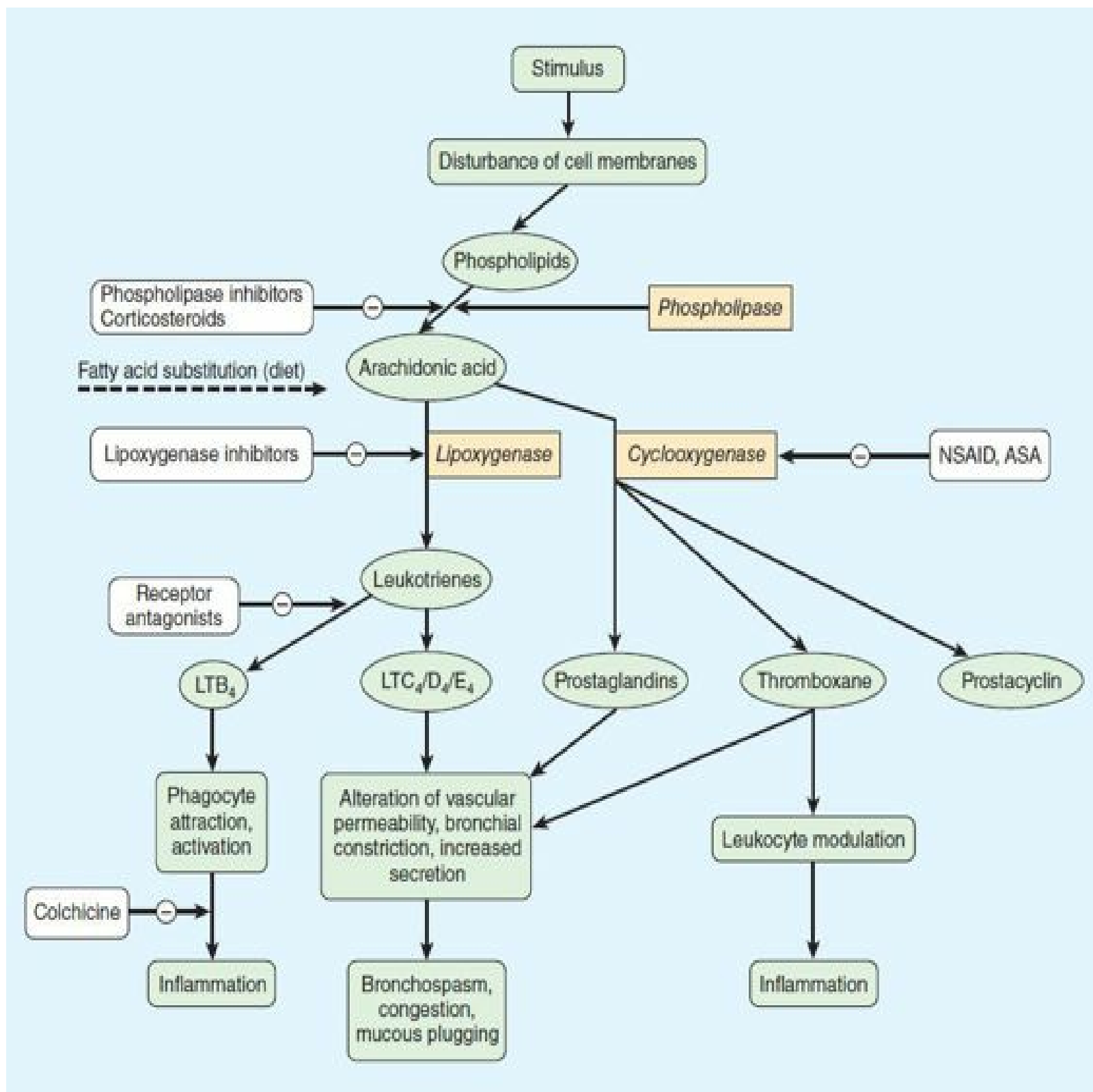
FIGURE 36–2 Prostanoid mediators derived from arachidonic acid and sites of drug action. ASA, acetylsalicylic acid (aspirin); LT, leukotriene; NSAID, nonsteroidal anti-inflammatory drug.
