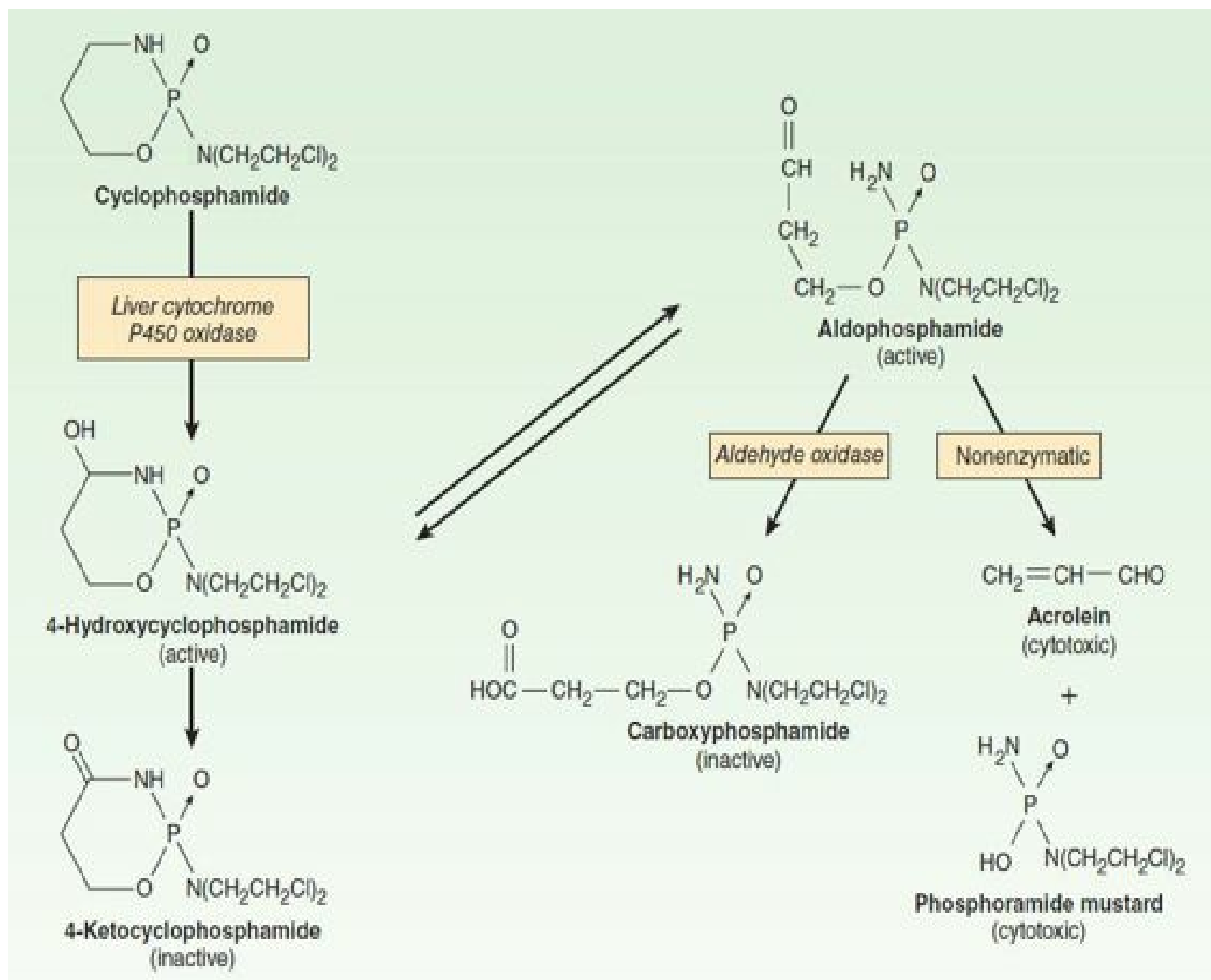
FIGURE 54–5 Cyclophosphamide metabolism.
