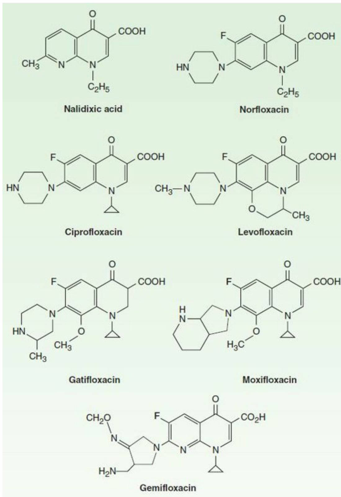
FIGURE 46–3 Structures of nalidixic acid and some fluoroquinolones.
