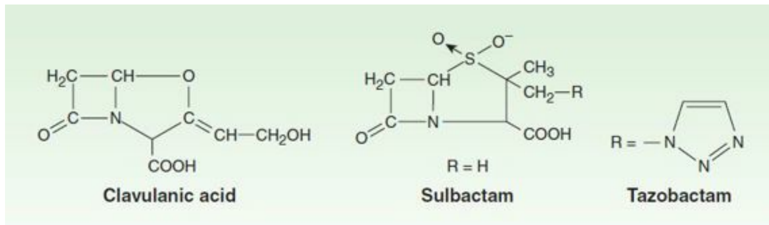
FIGURE 43–7 Beta-lactamase inhibitors.
