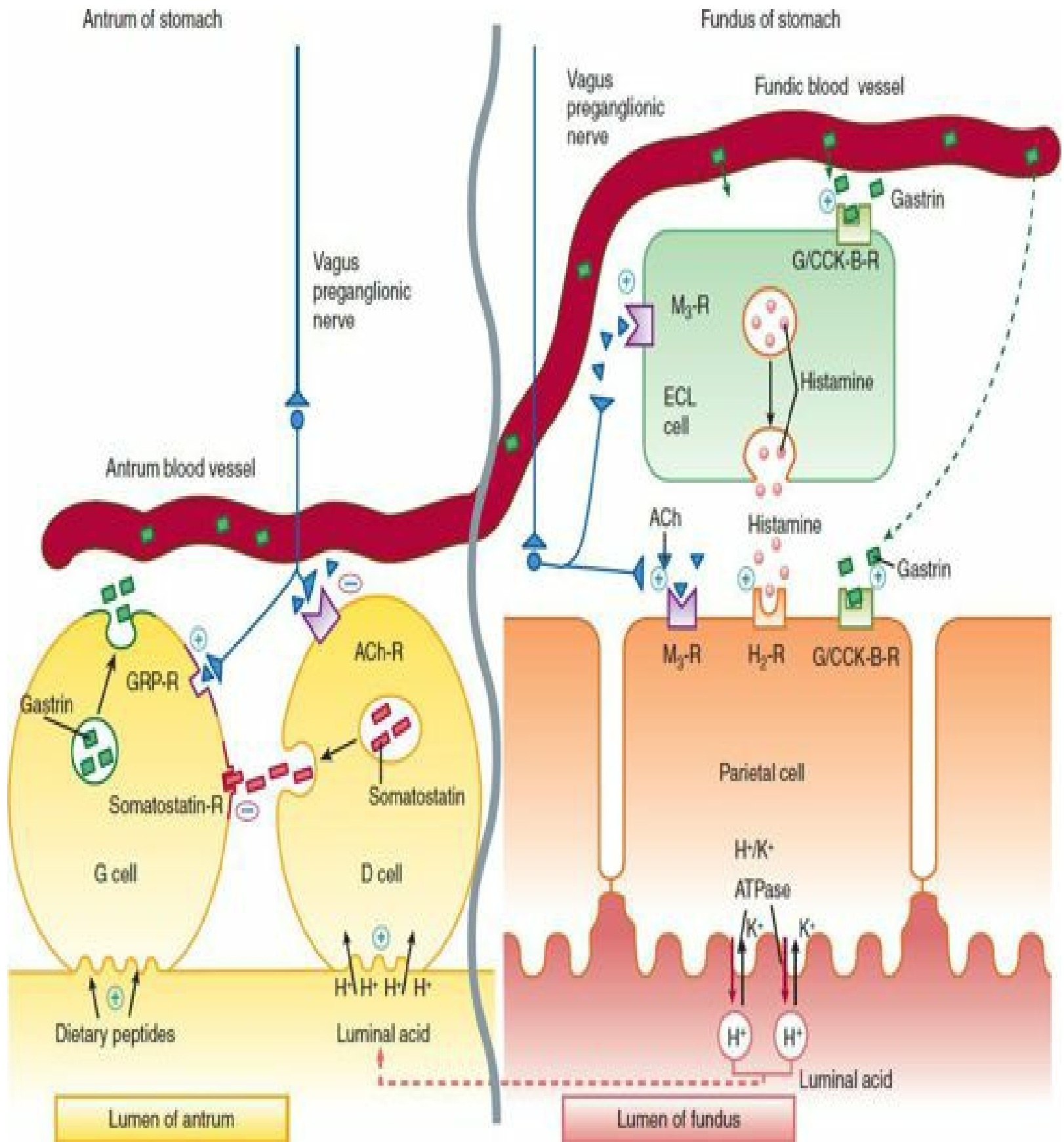
FIGURE 62–1 Schematic model for physiologic control of hydrogen ion (acid) secretion by the parietal cells of the gastric fundic glands. Parietal cells are stimulated to secrete acid ( H^+ ) by gastrin (acting on gastrin/CCK-B receptor), acetylcholine ( M_3 receptor), and histamine ( H_2 receptor). Acid is secreted across the parietal cell canalicular membrane by the H^+/K^+ -ATPase proton pump into the gastric lumen. Gastrin is secreted by antral G cells into blood vessels in response to intraluminal dietary peptides. Within the gastric body, gastrin passes from the blood vessels into the submucosal tissue of the fundic glands, where it binds to gastrin-CCK-B receptors on parietal cells and enterochromaffin-like (ECL) cells. The vagus nerve stimulates postganglionic neurons of the enteric nervous system to release acetylcholine (ACh), which binds to M_3 receptors on parietal cells and ECL cells. Stimulation of ECL cells by gastrin (CCK-B receptor) or acetylcholine ( M_3 receptor) stimulates release of histamine. Within the gastric antrum, vagal stimulation of postganglionic
