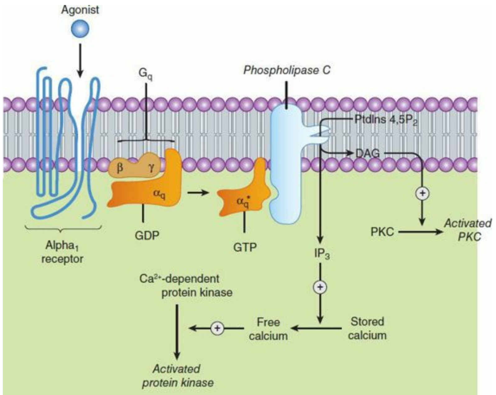
FIGURE 9-1 Activation of \alpha_1 responses. Stimulation of \alpha_1 receptors by catecholamines leads to the activation of a G_q -coupling protein. The activated \alpha subunit ( \alpha_q ) of this G protein activates the effector, phospholipase C, which leads to the release of IP 3 (inositol 1,4,5-trisphosphate) and DAG (diacylglycerol) from phosphatidylinositol 4,5-bisphosphate (PtdIns 4,5P 2 ). IP 3 stimulates the release of sequestered stores of calcium, leading to an increased concentration of cytoplasmic Ca 2+ . Ca 2+ may then activate Ca 2+ -dependent protein kinases, which in turn phosphorylate their substrates. DAG activates protein kinase C (PKC). GTP, guanosine triphosphate; GDP, guanosine diphosphate. See text for additional effects of \alpha_1 -receptor activation.
