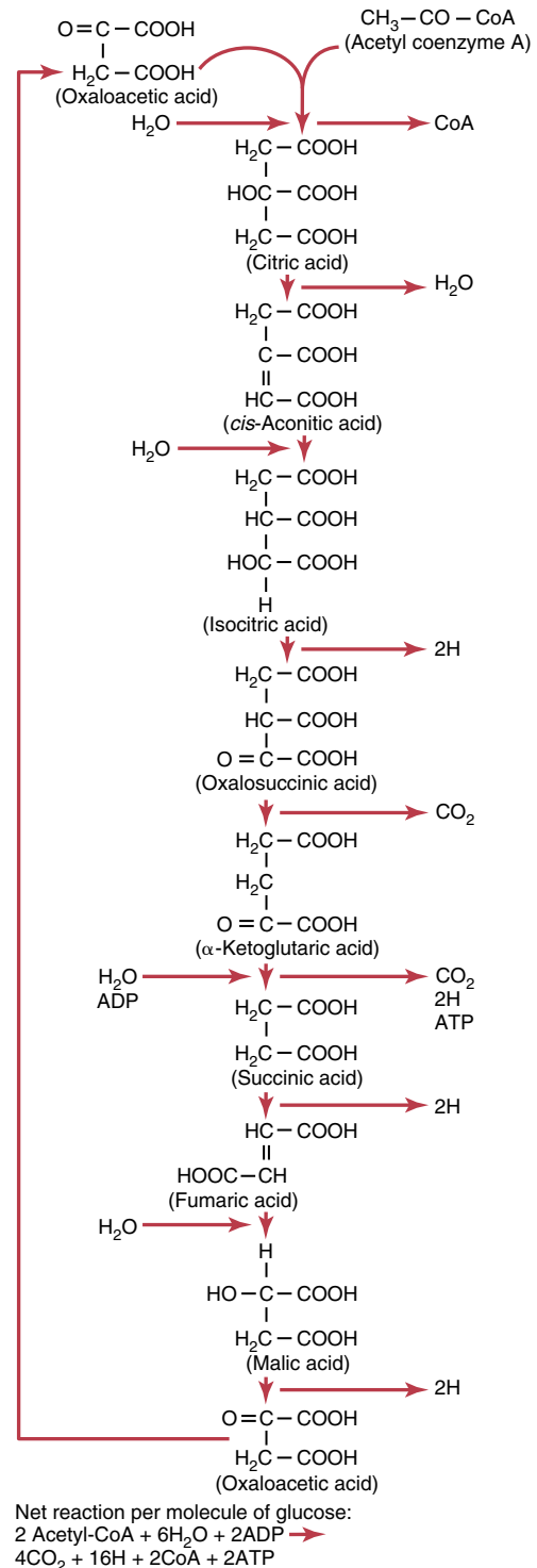
Figure 68-6. Chemical reactions of the citric acid cycle, showing the release of carbon dioxide and a number of hydrogen atoms during the cycle. ADP, Adenosine diphosphate; ATP, adenosine triphosphate.
